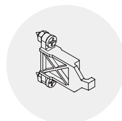
TEMPLATE TO FIX THE CLIP OF THE DRAWER FRONT
