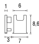
601T004 Tappi (opzionali) Terminals (optional) / Verschlüsse (optional)
