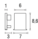
601T004C Tappi chiusi (opzionali) Closed terminals (optional) / Verschlüsse (optional)
