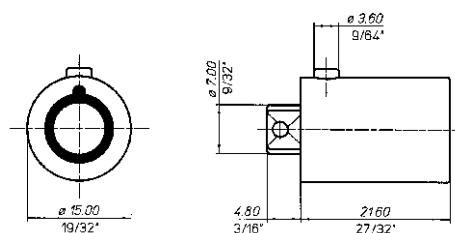
Nucleo con autoaggancio Nucleo with self-fixing
