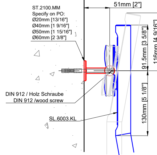
Detail Z
