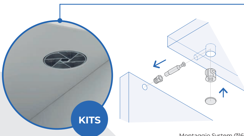
Montaggio System Ø16 Assembling System
