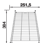
FLOATING GRID
